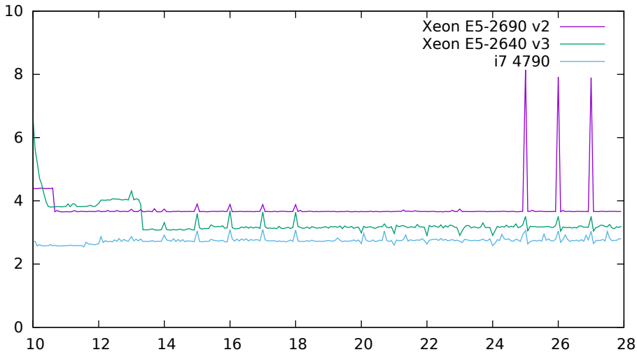
sequential memory access time vs. stride (8 accesses)
