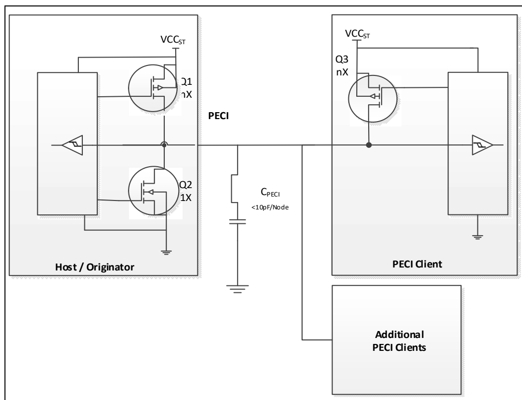
Figure 2-1. Example for PECI Host-Clients Connection
