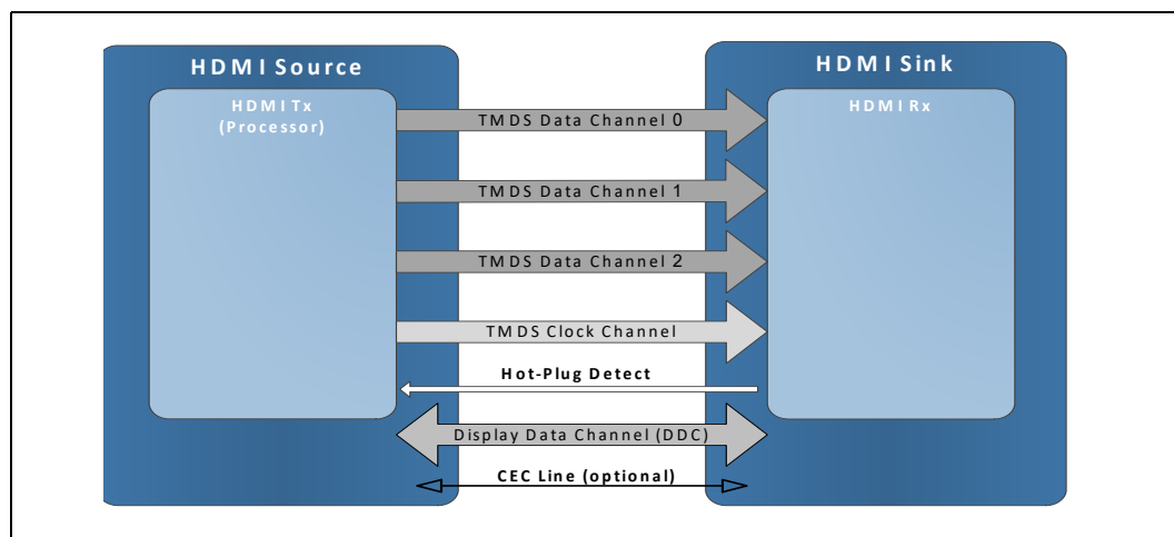
Figure 10-3. HDMI* Overview
