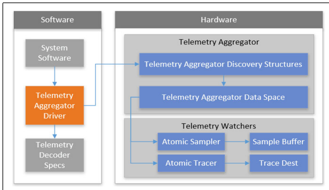
Figure 2-6. Telemetry Aggregator
