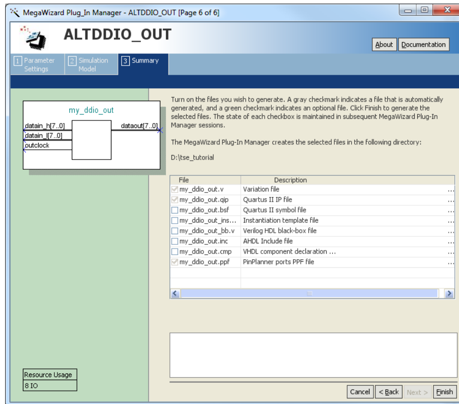
Figure 18. Settings for the Summary tab of DDIO_OUT register.
