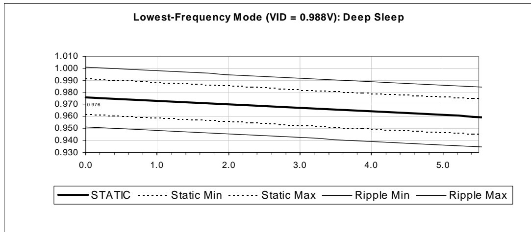
Figure 3-8. Illustration of Deep Sleep State V CC Static and Ripple Tolerances (LFM- VID#D)
