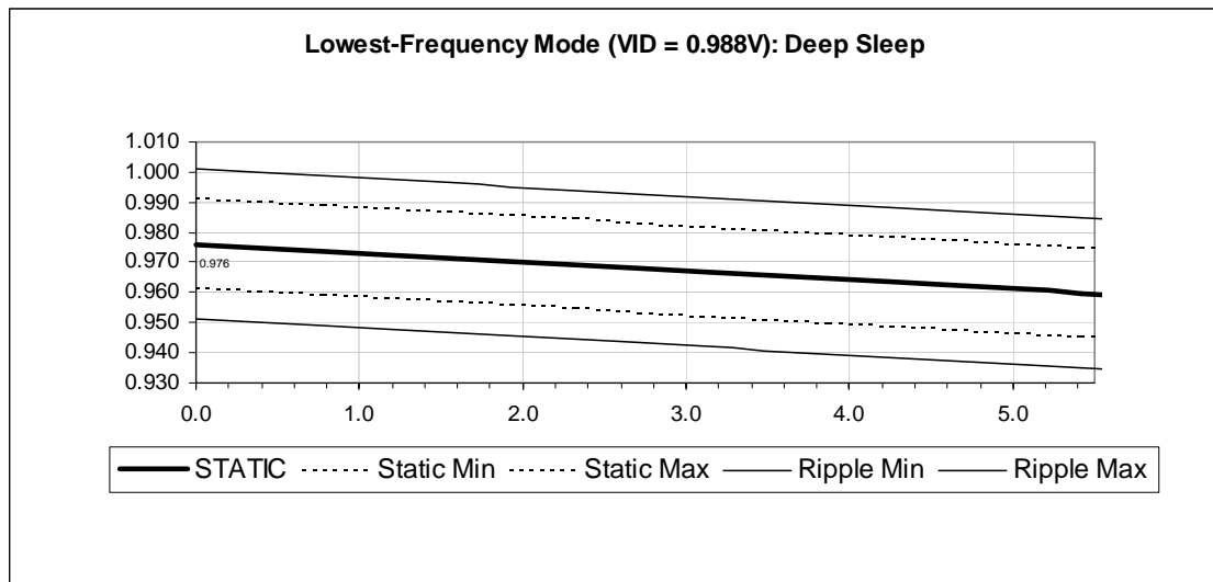
Figure 3-6. Illustration of Deep Sleep State V CC Static and Ripple Tolerances (LFM- VID#C)
