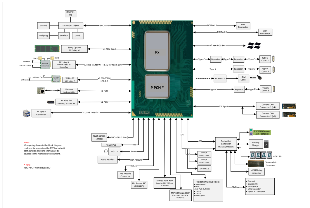
Figure 4. PX Processor Line Platform Diagram
