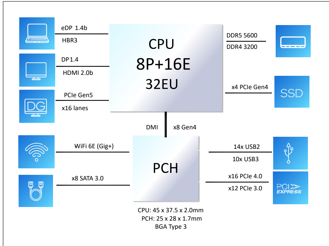
Figure 4. PX Processor Line Platform Diagram
