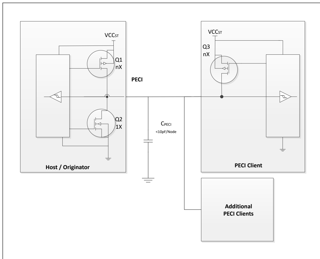
Figure 5. Example for PECCI Host-Clients Connection
