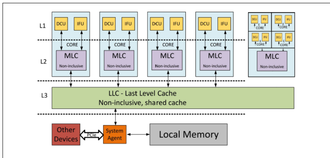
Figure 8. Hybrid Cache
