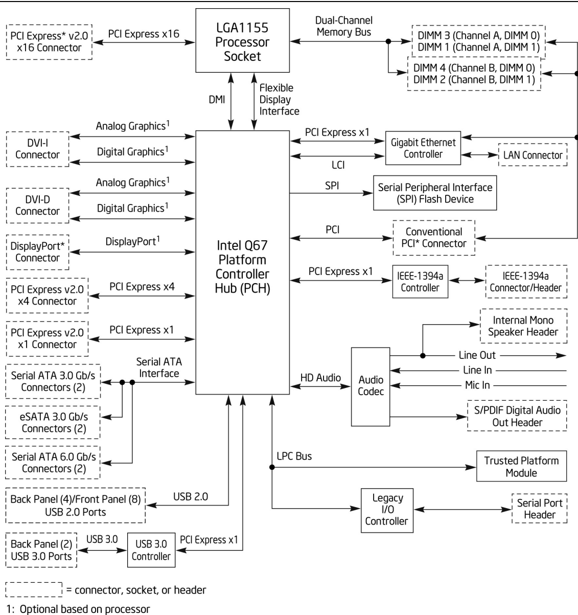
Figure 2 is a block diagram of the major functional areas of the board.
