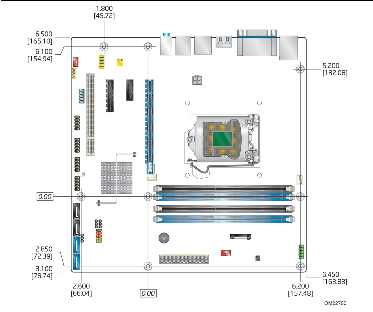
Figure 15. Board Dimensions
