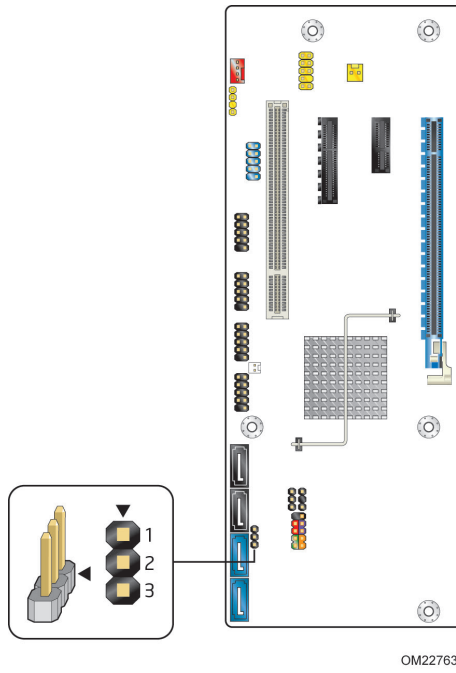
Figure 14. Intel MEBX Reset Header
