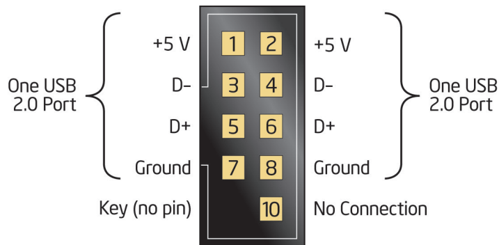
Figure 12. Connection Diagram for Front Panel USB 2.0 Connectors
