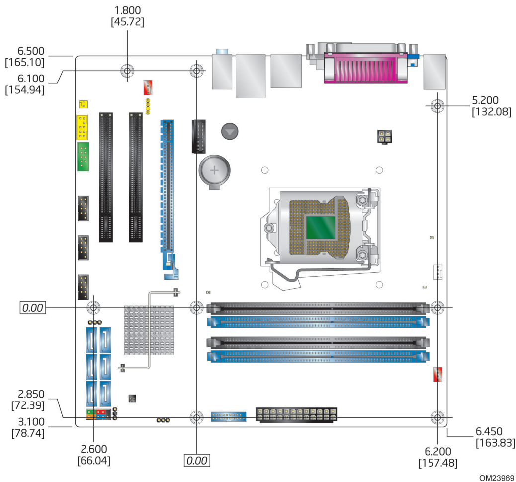
Figure 16. Board Dimensions
