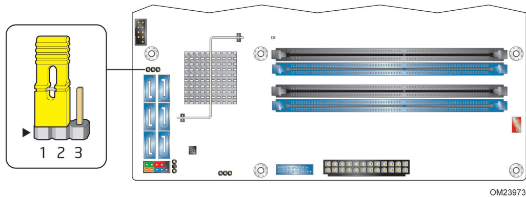
Figure 14. Location of the Jumper
