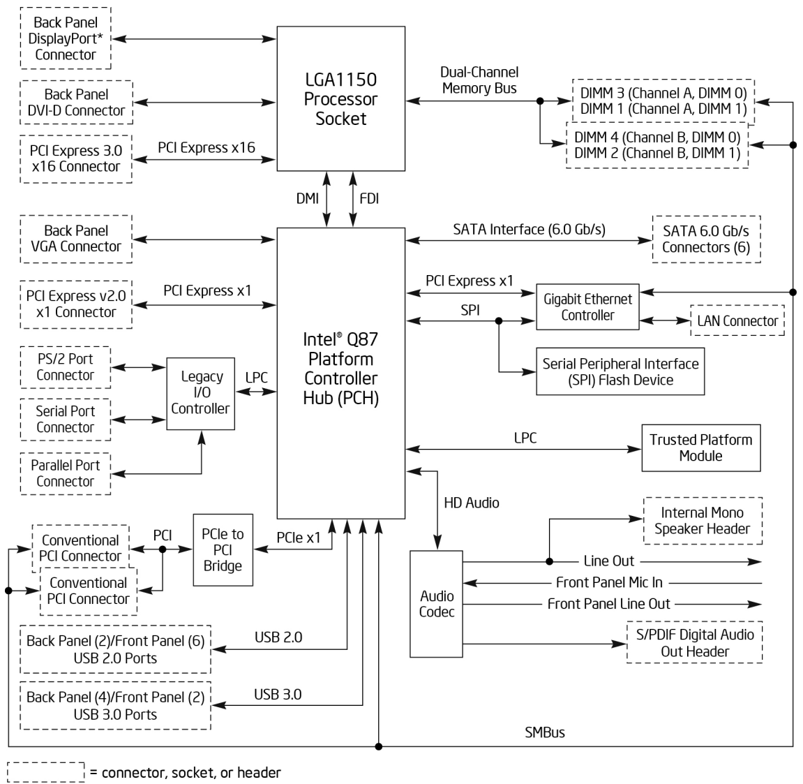
Figure 2. Block Diagram
