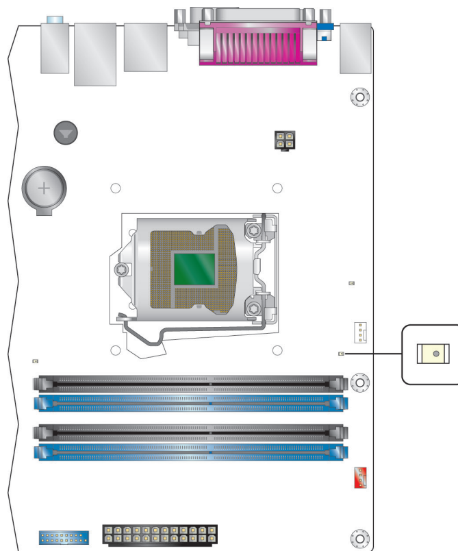
Figure 8. Location of the Enhanced Standby Power LED
