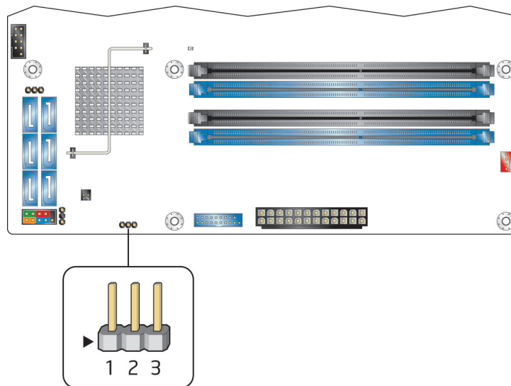
Figure 15. Intel MEBX Reset Header
