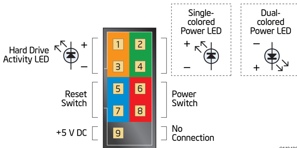
Figure 11. Connection Diagram for Front Panel Connector
