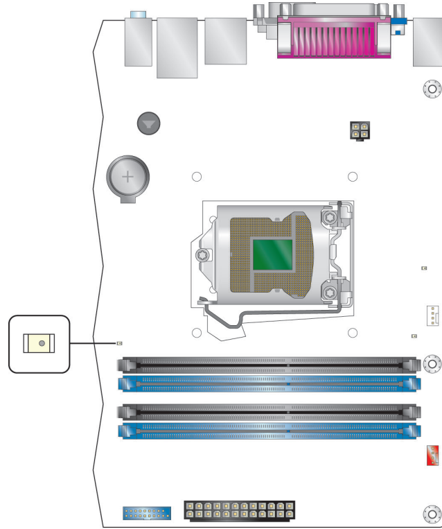
Figure 7. Location of the Intel ME "M" State LED
