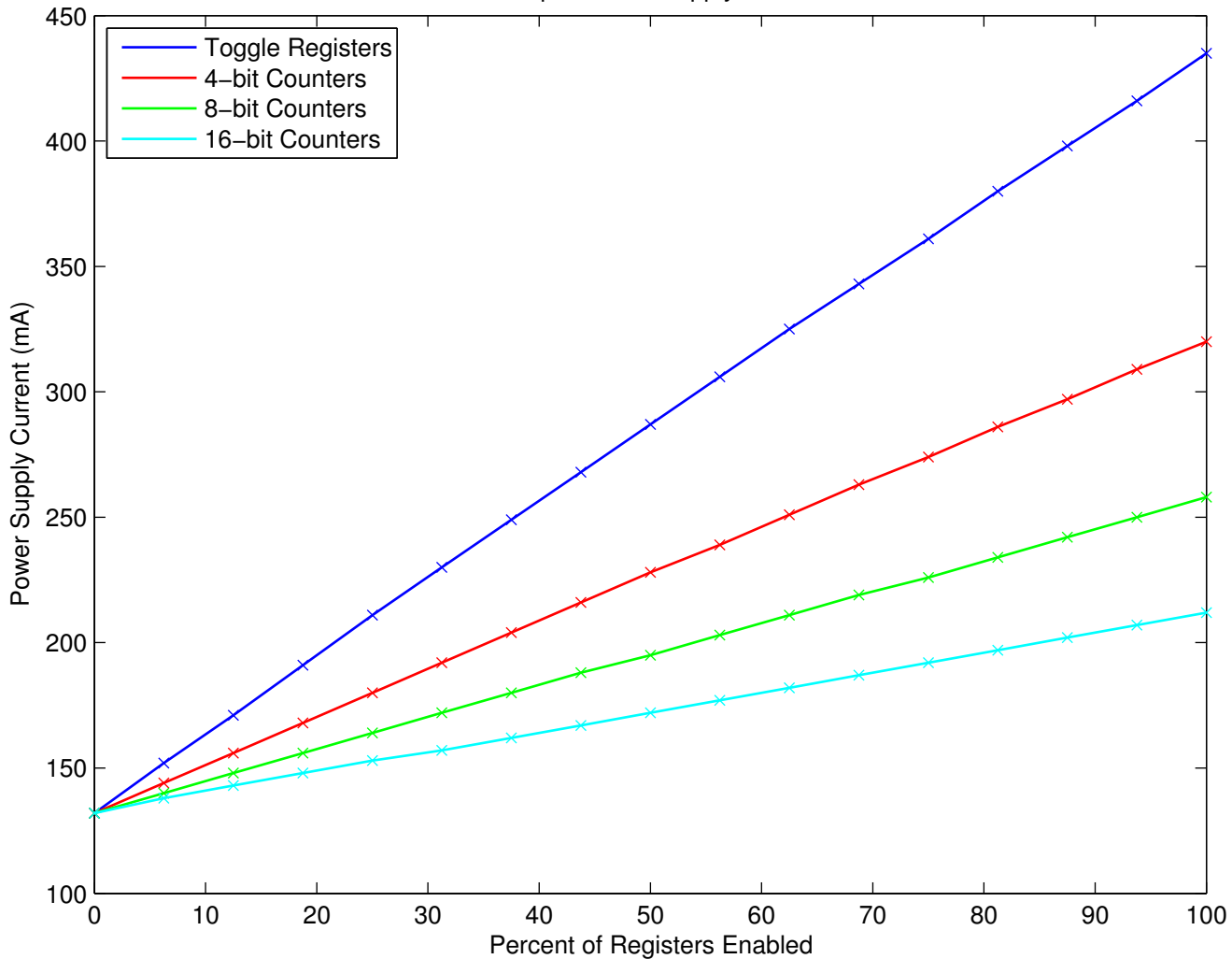
DE0-nano Input Power Supply Measurements
