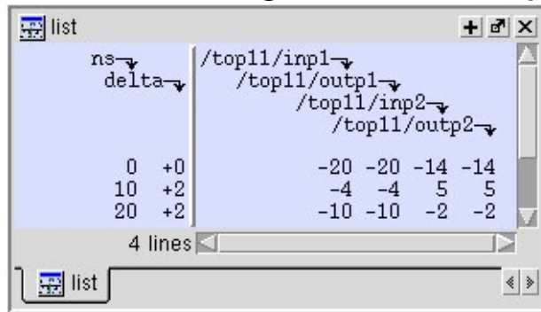
Figure 4-28. List Window After configure list -delta collapse Option is Used
