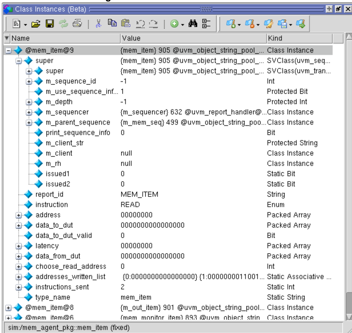
Figure 4-7. Class Instances Window
