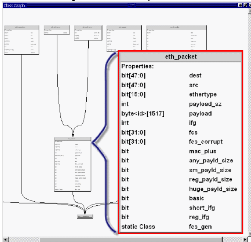
Figure 4-6. Class Graph Window
