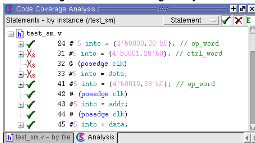
Figure 4-9. Code Coverage Analysis
