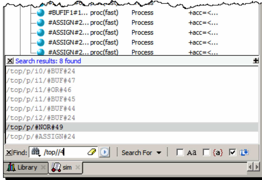
Figure 1-10. Find Mode Popup Displaying Matches
