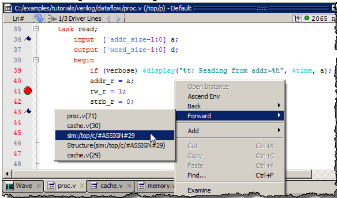
Figure 4-69. Setting Context from Source Files
