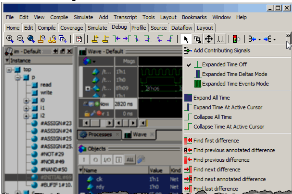
Figure 3-30. Toolbar Tabs and Overflow Menu
