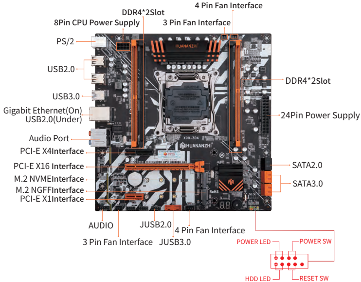
1-1 X99-ZD4 Motherboard Illustration
