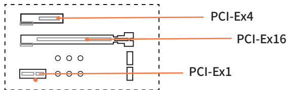
2-4 PCI-E Slot
