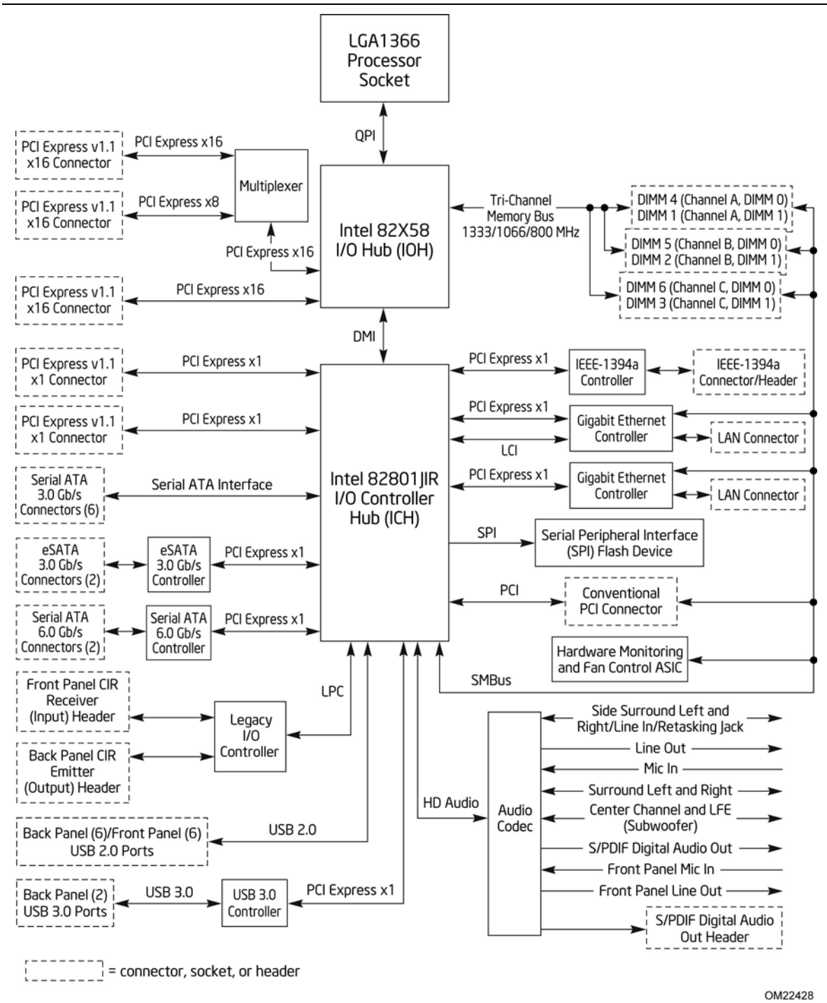
Figure 2. Block Diagram
