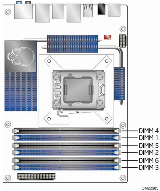
Figure 3. Memory Channel and DIMM Configuration
