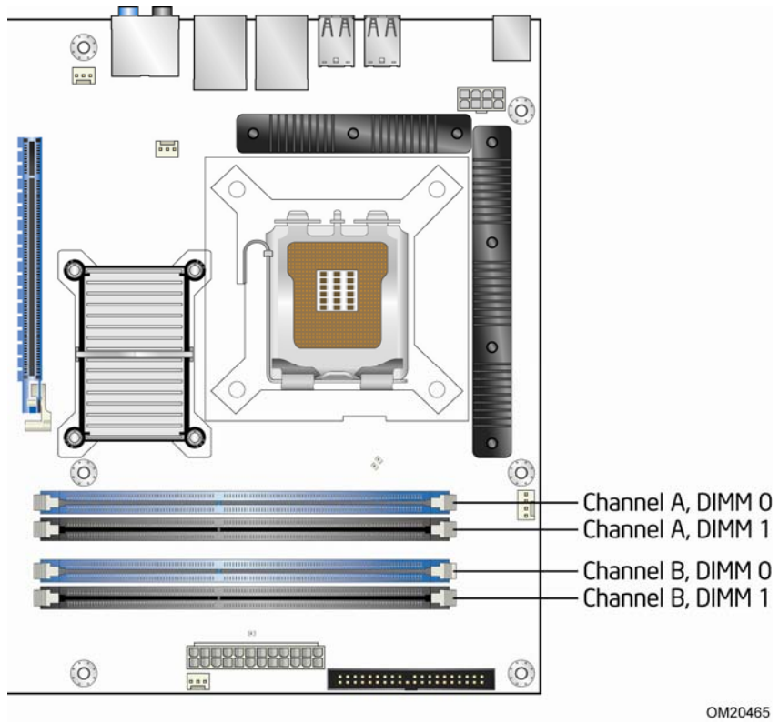
Figure 3. Memory Channel and DIMM Configuration
