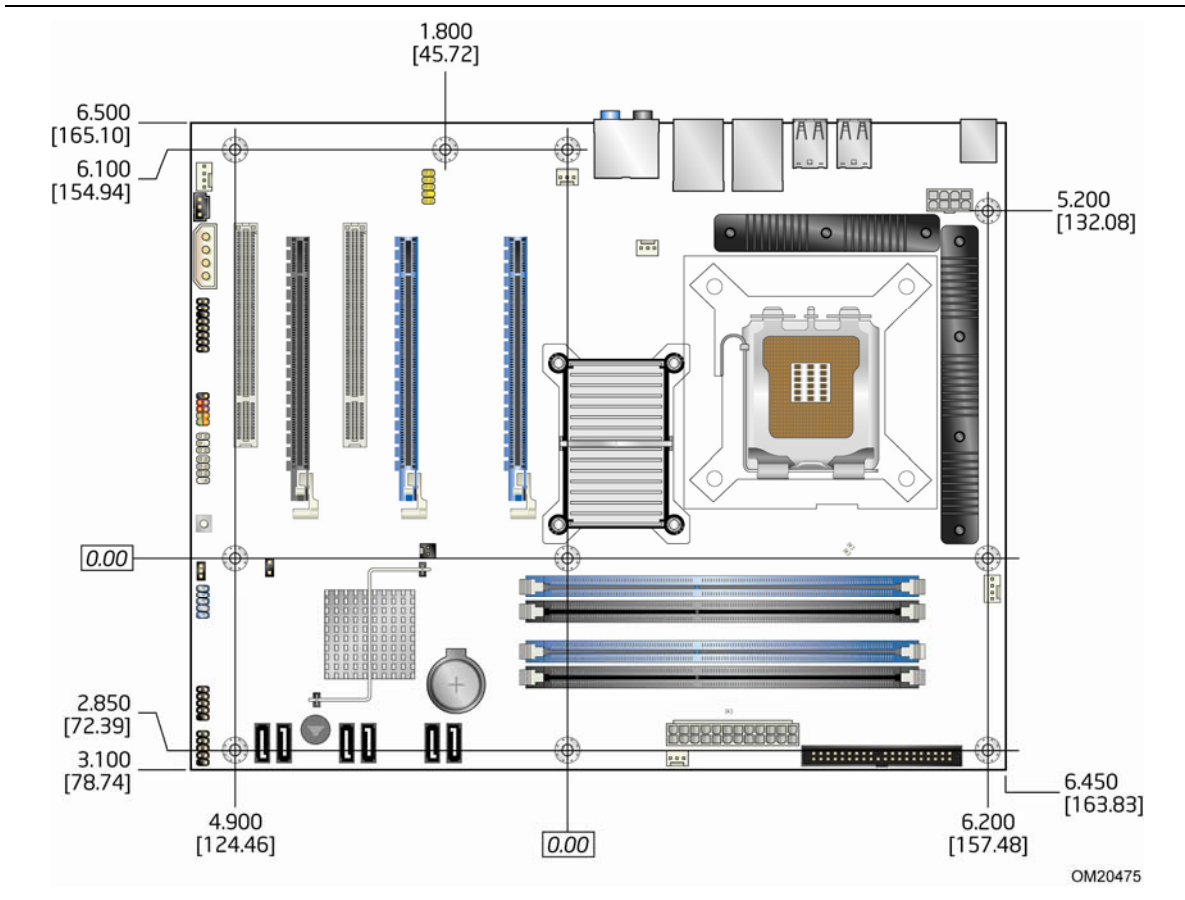
Figure 16. Board Dimensions
