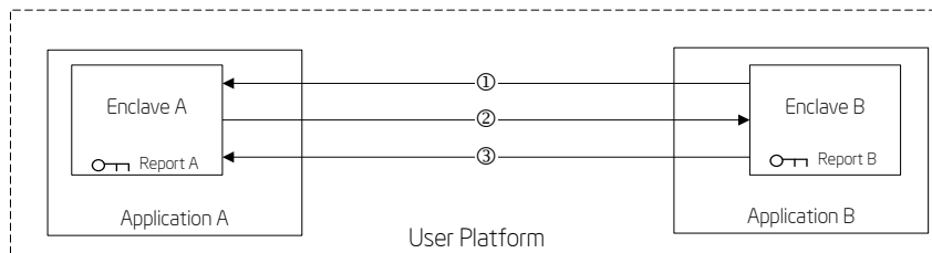
Figure 5-1 Local Attestation Example
