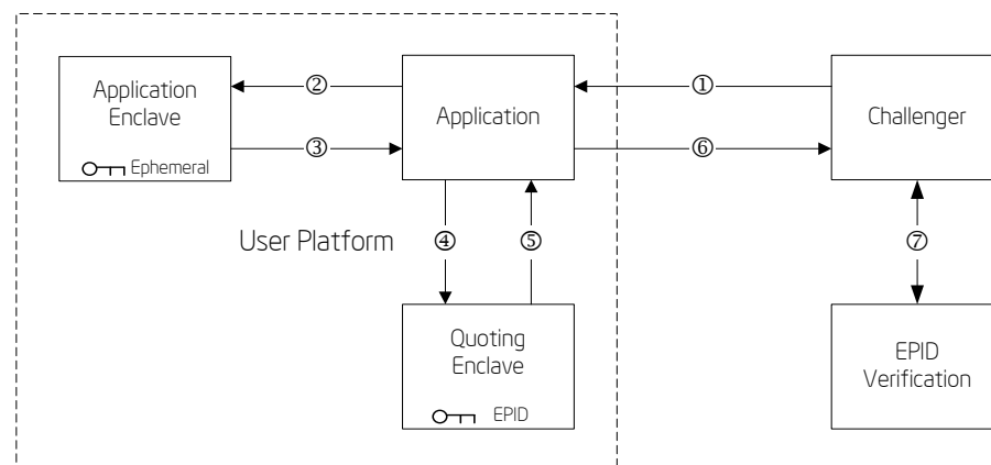
Figure 5-2 Remote Attestation Example
