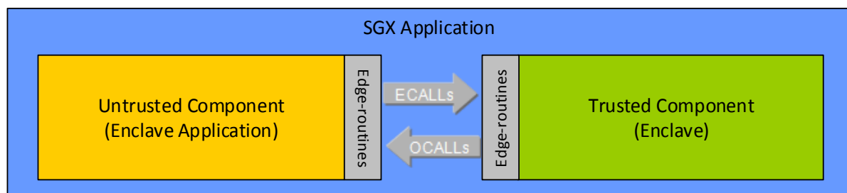
Figure 2-1 Intel® SGX Application
