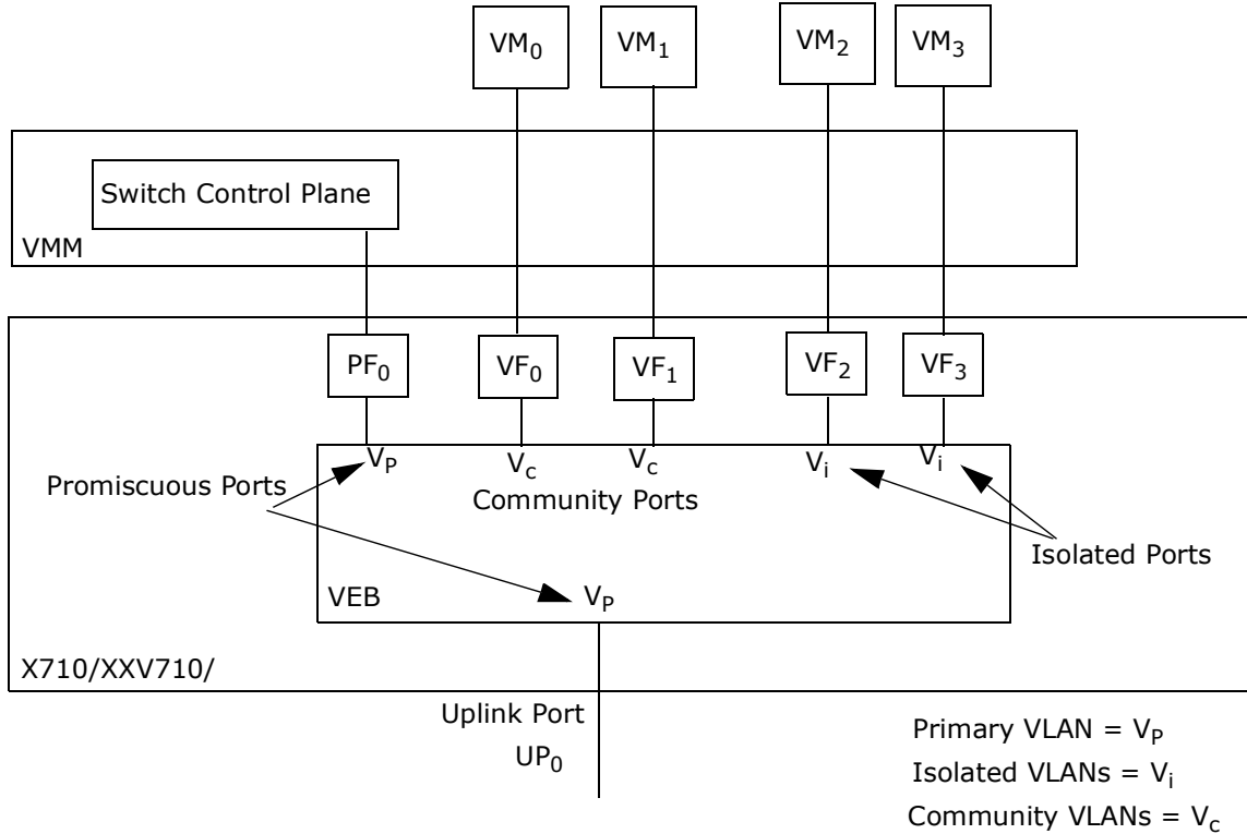
Figure 7-50. PVLAN configuration
