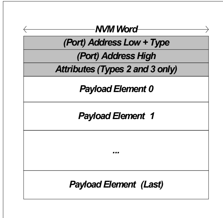
Figure 6-1. Structure of a flexible functionality module
