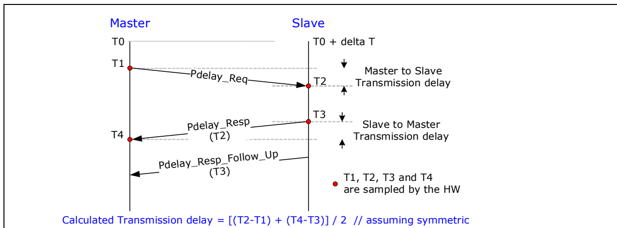
Figure 8-12. PDelay Flow
