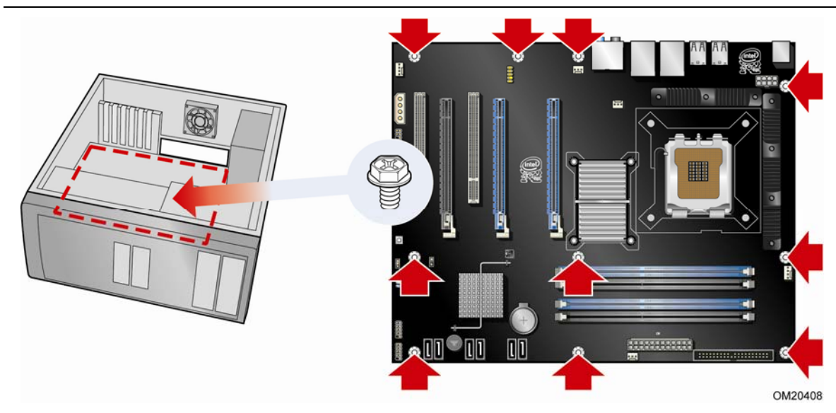
Figure 7. Desktop Board DX38BT Mounting Screw Hole Locations
