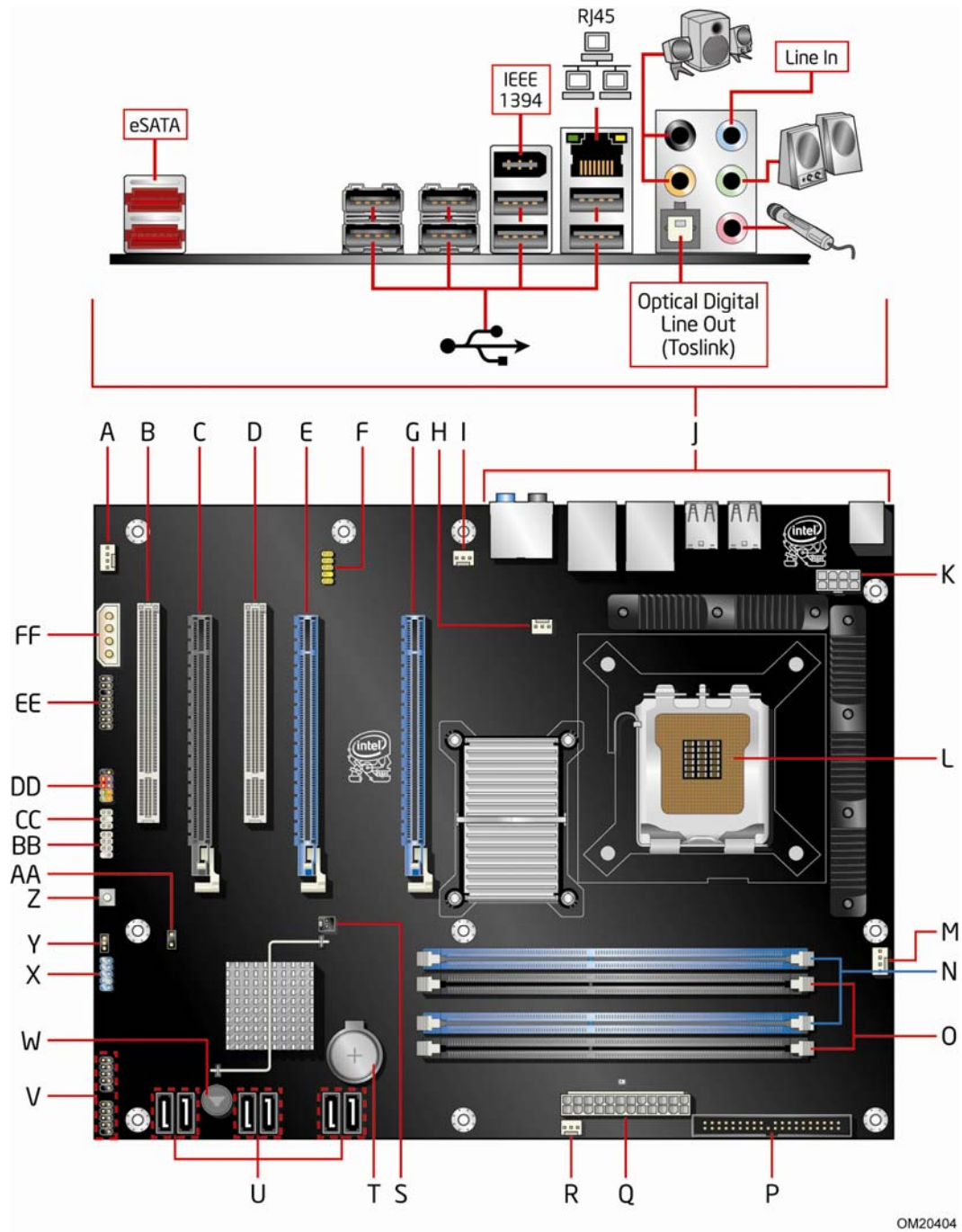
Figure 1. Desktop Board DX38BT Components
